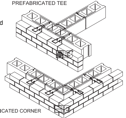
PREFABRICATED TEE
